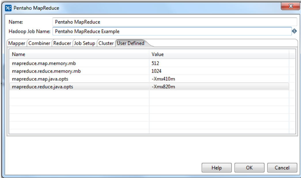
Figure 8: User Defined Tab
