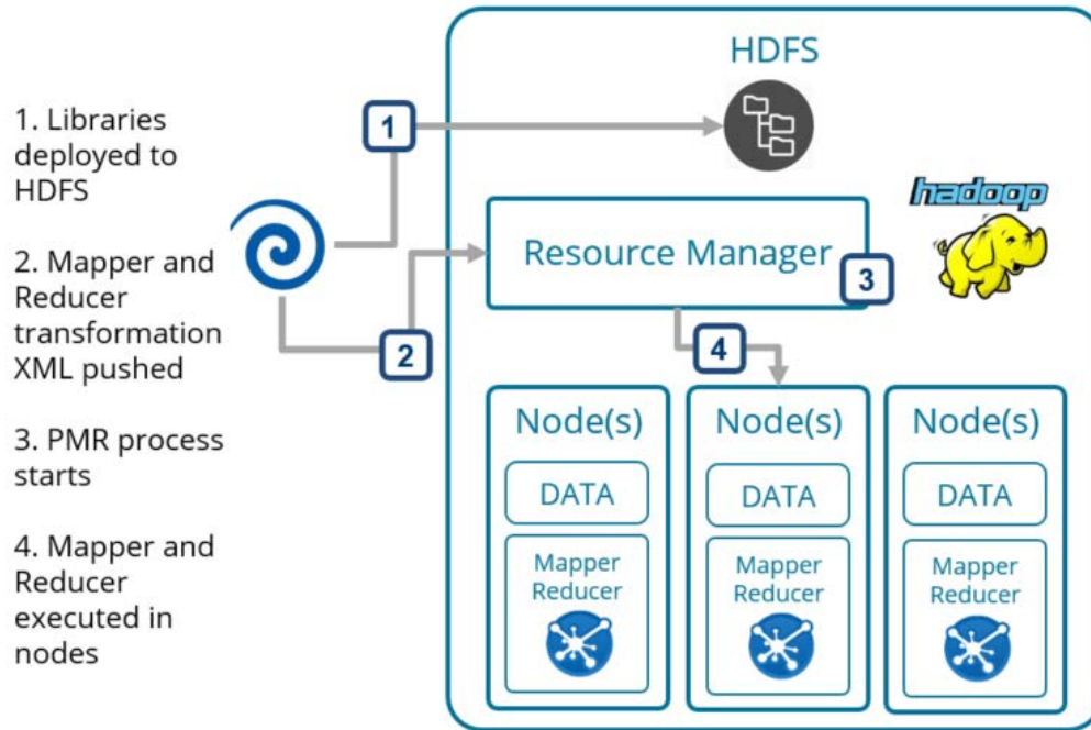
Figure 1: Executing PDI
